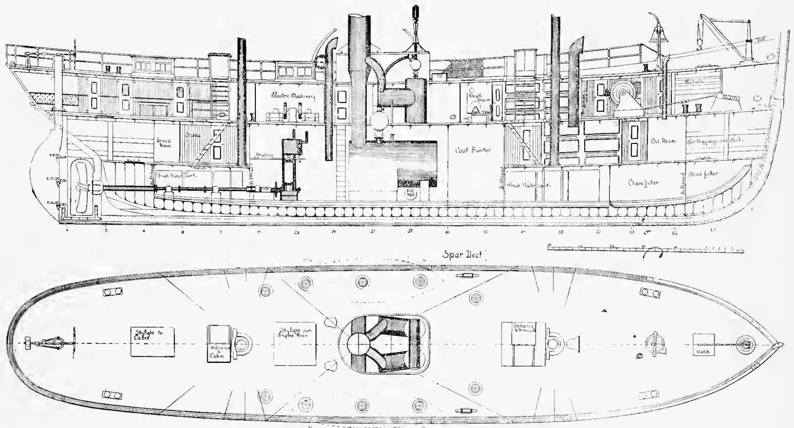
PLANS FOR A COMPOSITE STEAM LIGHT VESSEL FOR THE WOODS HOLE, (MASS.) STATION.
